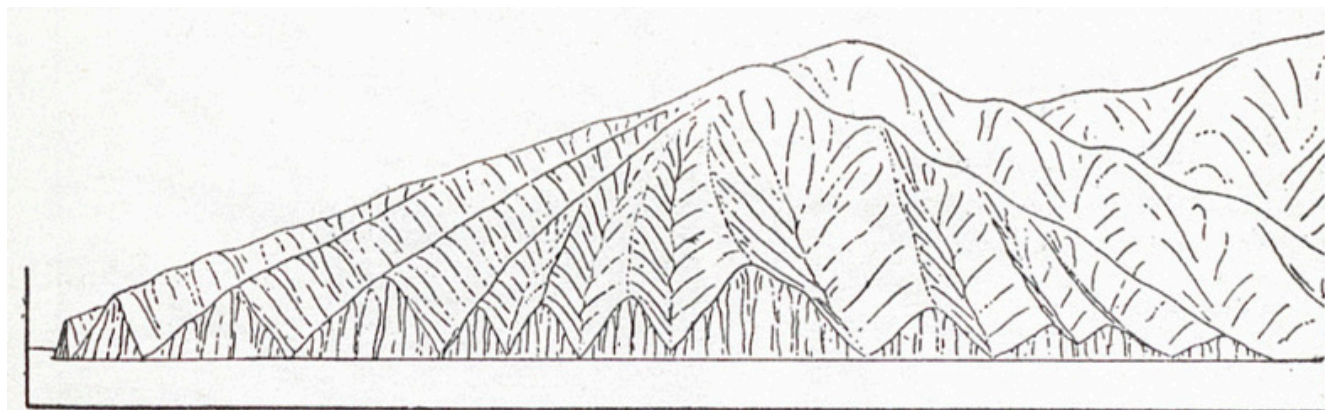
Fig. 18—Morne au Diable, a maturely dissected volcano at the northern end of Dominica.
