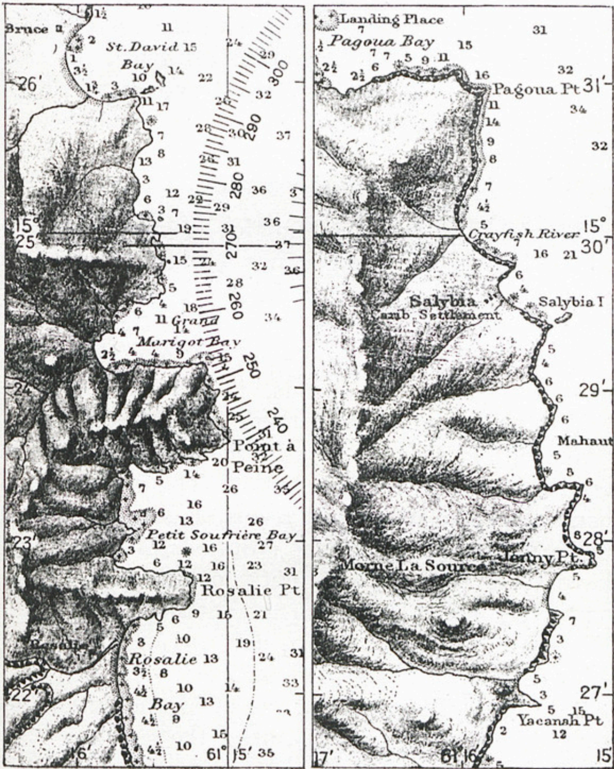
Fig. 21—An embayed and cliffed part of the east coast of Dominica (from U. S. Hydrogr. Office Chart No. 1318).
