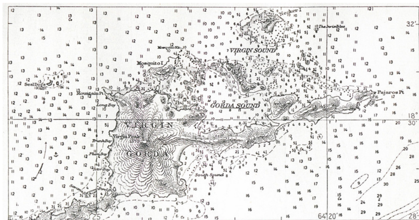
Fig. 45—The embayed island of Virgin Gorda (from U. S. Hydrogr. Office Chart No. 3904).
